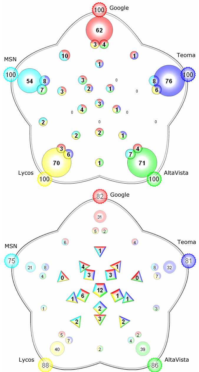
Figure 1: (Top) The Category View shows the overlap between the top 100 items found by Google, Teoma, AltaVista, Lycos & MSN, when searching for 'information visualization'. (Bottom) If a URL equal to the server address is used to match items, then the overlap increases. Icons for items retrieved by at least 3 engines are selected. Shape (size) coding is used for icons (not) selected.
