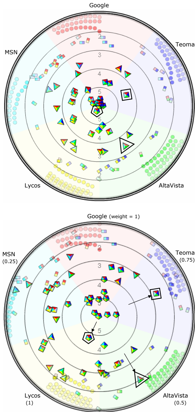
Figure 2: (Top) The Cluster Bulls-Eye View uses polar coordinates to place in close proximity documents with similar rankings by the different search engines. A document's radius is a function of the number of engines that retrieved it and the average of its different ranking scores. A document's angle reflects the relative ratio of its rankings by the different engines. (Bottom) Shows how all the documents cluster if the engines are assigned different weights of importance (1, 0.75, 0.5, 1, 0.25) and the radius is now equal to the weighted average of the rankings by the different engines. In both displays, the documents found by at least three engines are selected. Three documents are highlighted to show how their locations change when the weights are applied.
