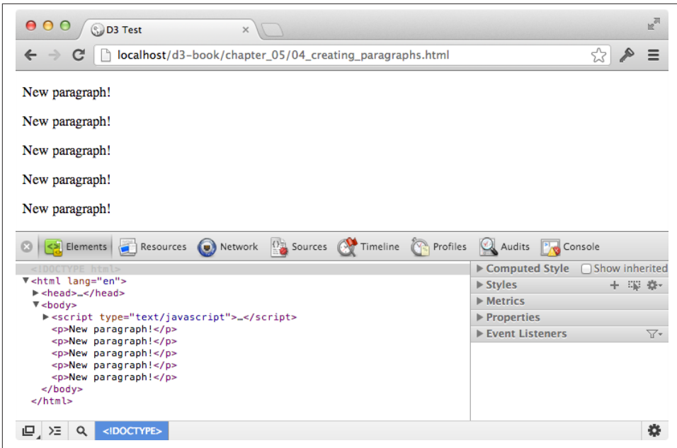
Figure 5-6. New p elements in the web inspector
