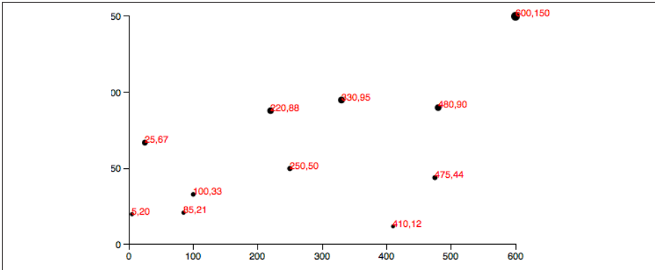
Figure 8-6. Initial y-axis
