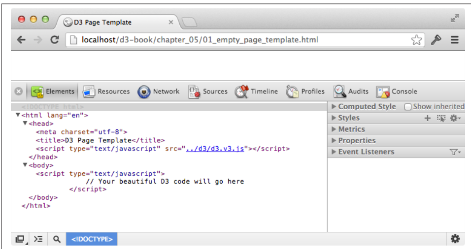
Figure 5-1. Web inspector
