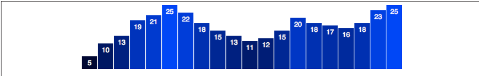
Figure 6-31. Centered labels
