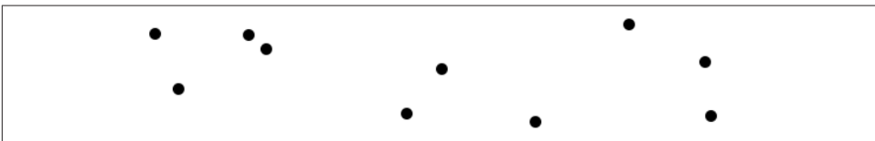
Figure 6-32. Simple scatterplot
