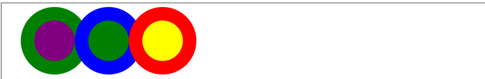
Figure 3-25. Opaque circles
