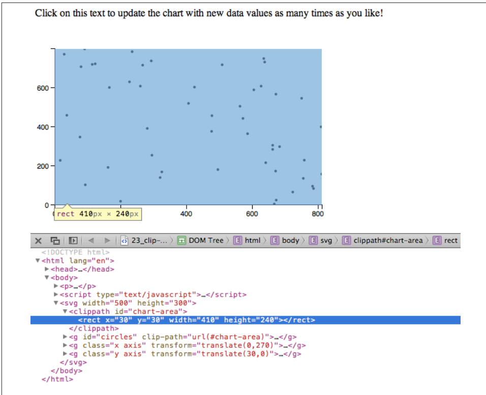
Figure 9-15. The dimensions of a rect within a clipPath
