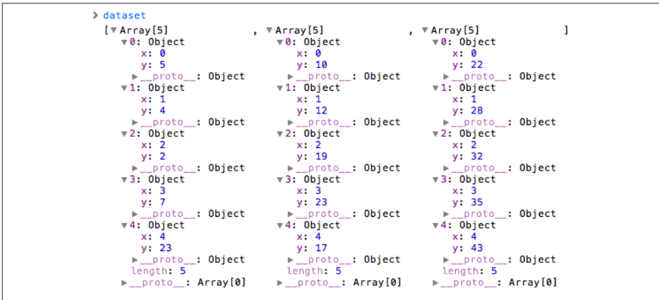
Figure 11-5. The data before stacking
