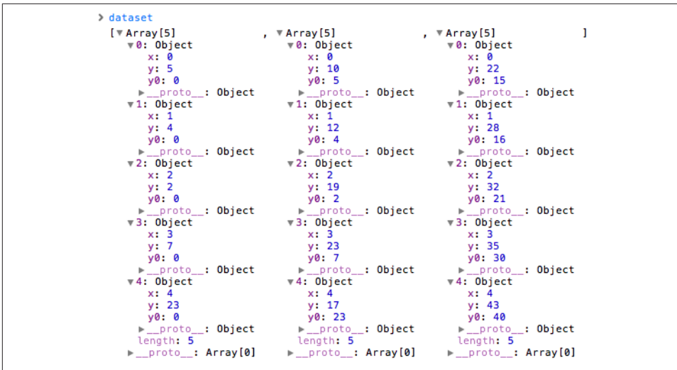
Figure 11-6. The data after stacking
