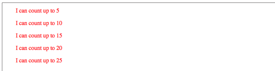
Figure 5-13. Red paragraphs
