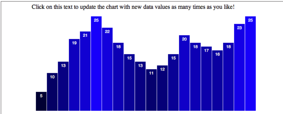
Figure 9-7. Initial view
