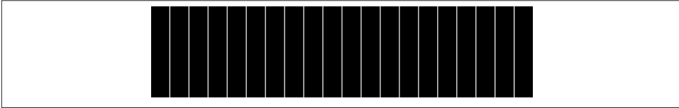
Figure 6-15. Twenty bars
