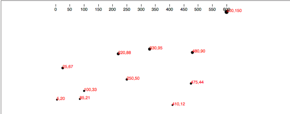
Figure 8-3. Cleaner axis
