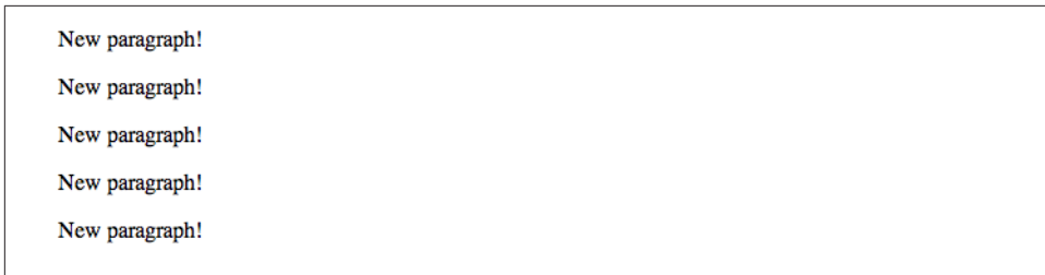
Figure 5-5. Dynamic paragraphs
