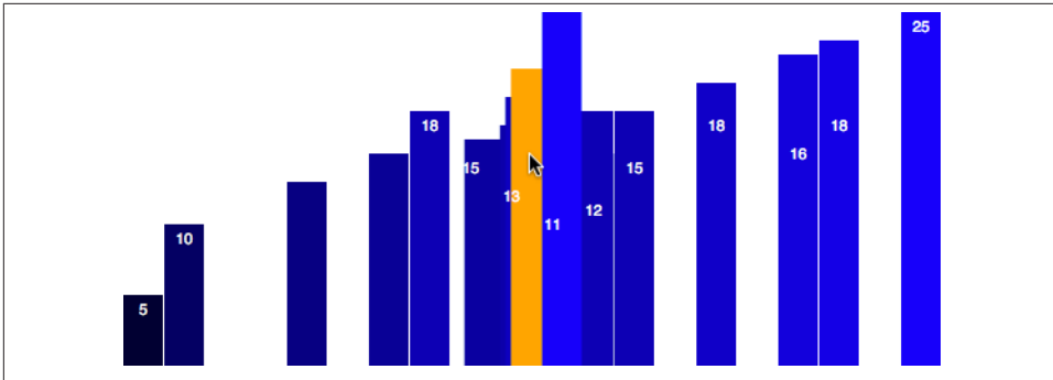
Figure 10-6. Transitions, interrupted
