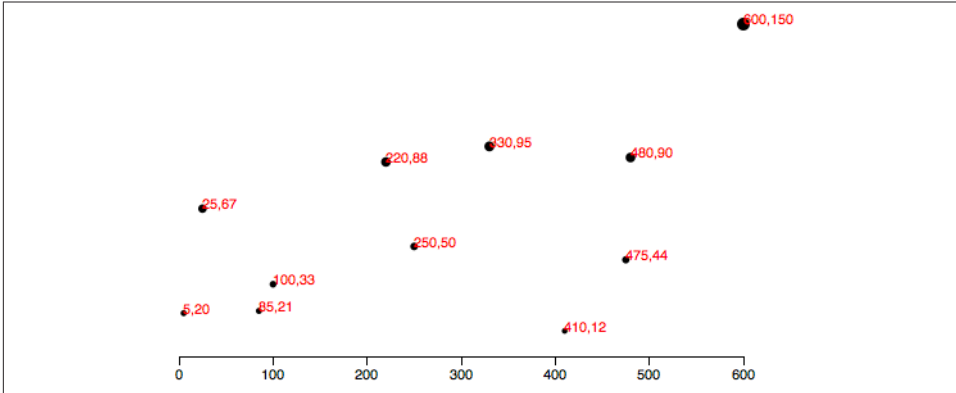
Figure 8-5. Fewer ticks
