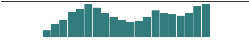
Figure 6-26. Teal bars
